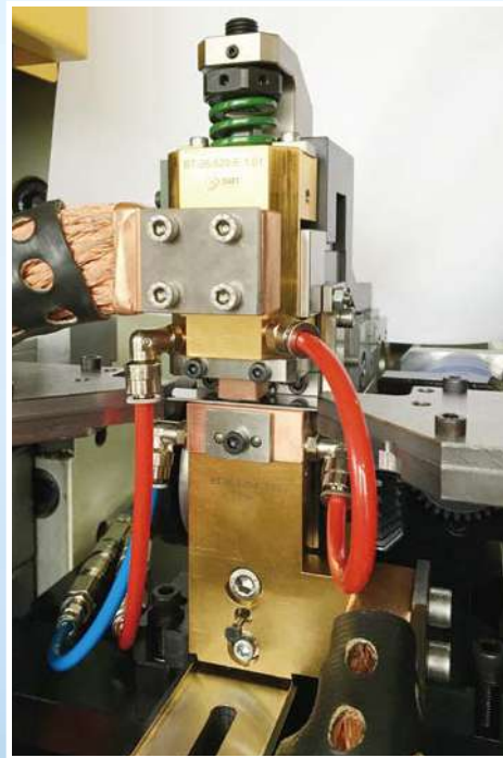
結合焊接機加工 Intergrated Welding Attachment
